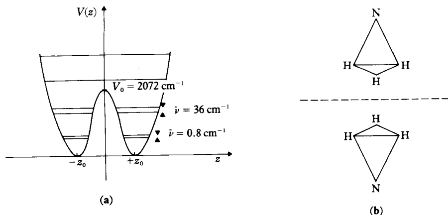
10.17 The potential well (a) for the inversion motion (b) of ammonia.
